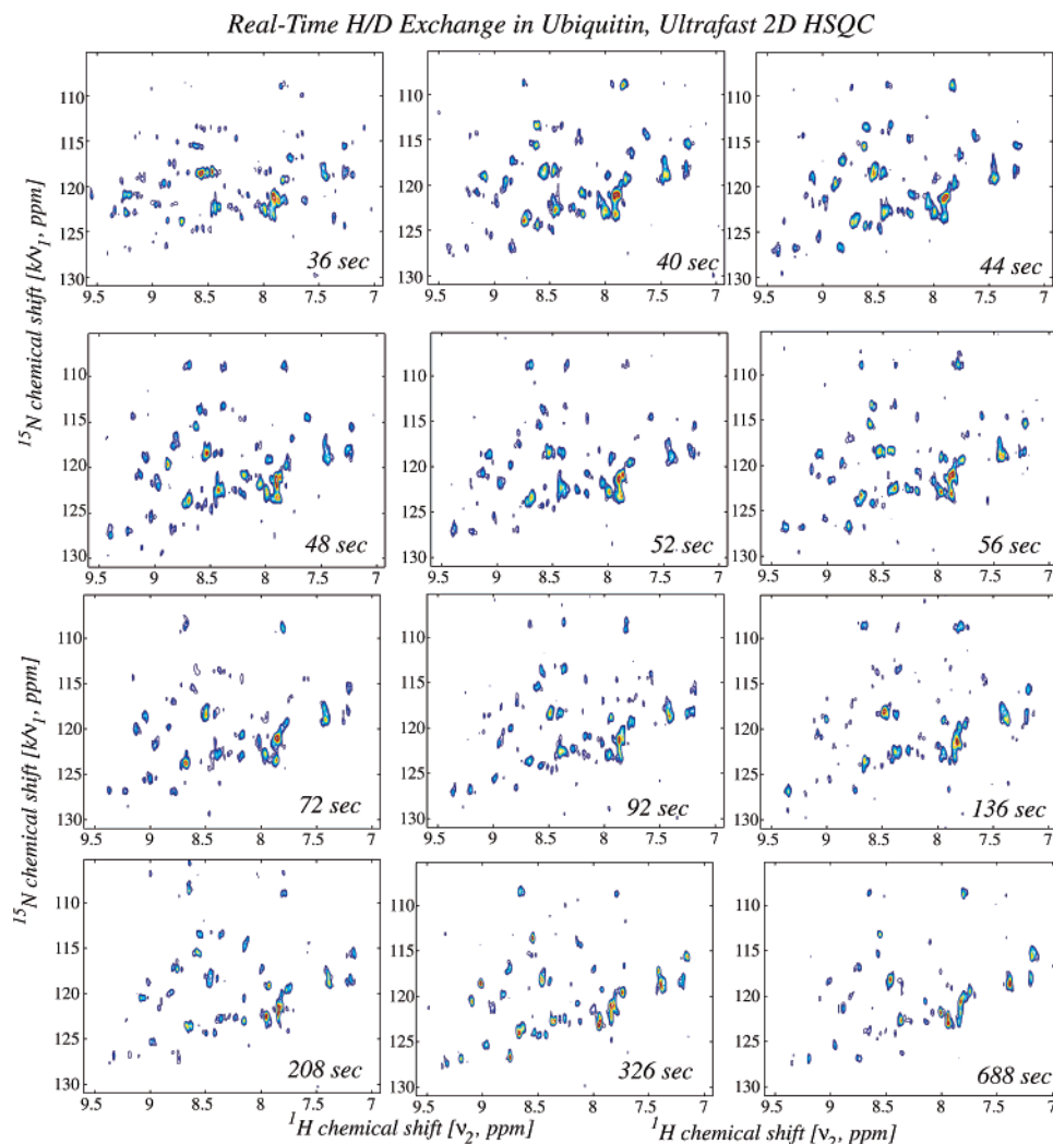
Figure 3. Representative series of real-time 2D HSQC NMR spectra recorded on a \sim 3.2 mM ubiquitin solution, following the dissolution of an initially fully protonated lyophilized powder onto a D_2O -based 50 mM phosphate buffer. The times indicated in each frame correspond to the approximate delay elapsed since the powder was initially dissolved (something which happened outside the magnet) and the average time of the data acquisition. In the actual experiment a full series of spectra separated by \sim 4 s was recorded over a 20 min interval; only a subset of these spectra is shown.
